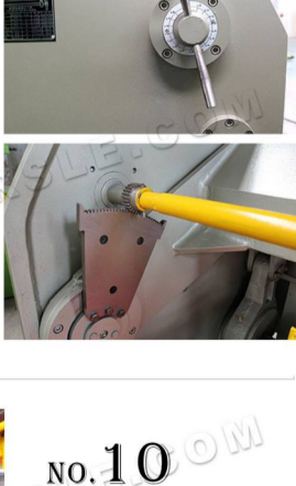
No. 9 Manual Knife Clearance Adjustment
